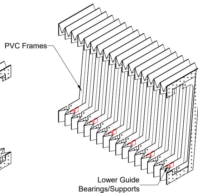
Isometric Rear View
