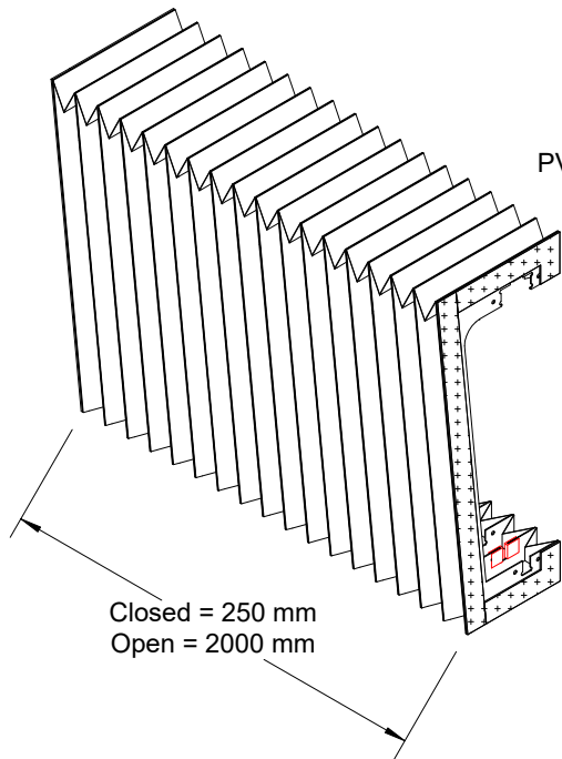
Isometric Front View
